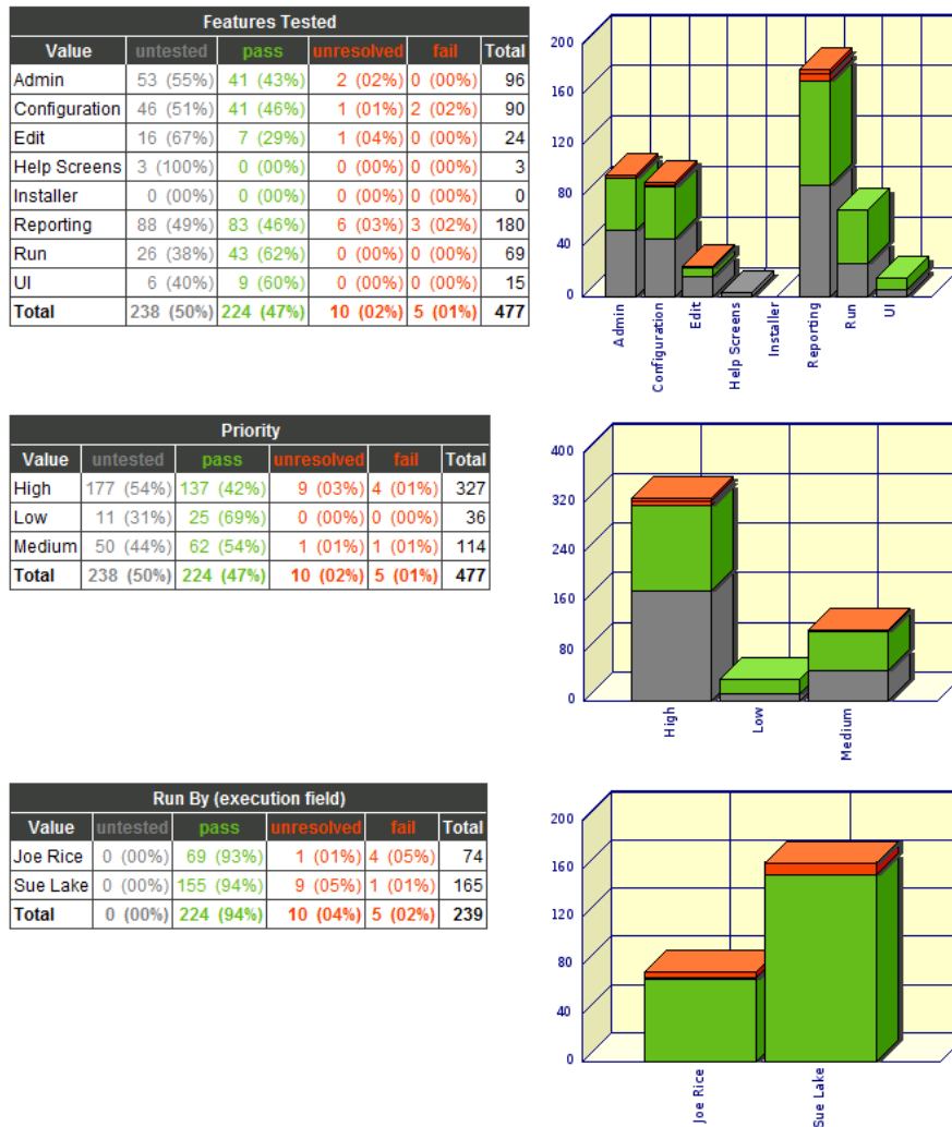
Figure 20 - Selector Summary Tables
