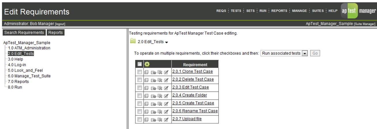
Figure 13 - Requirements tree
