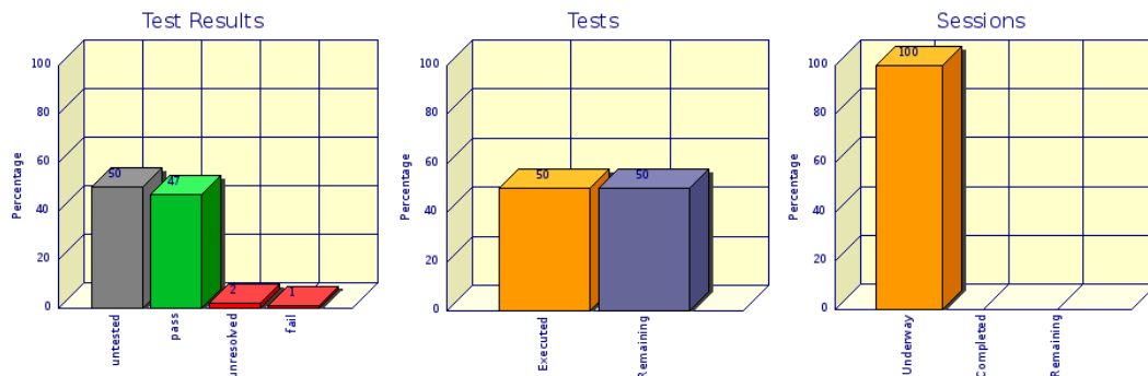
Figure 11 - Progress Report
