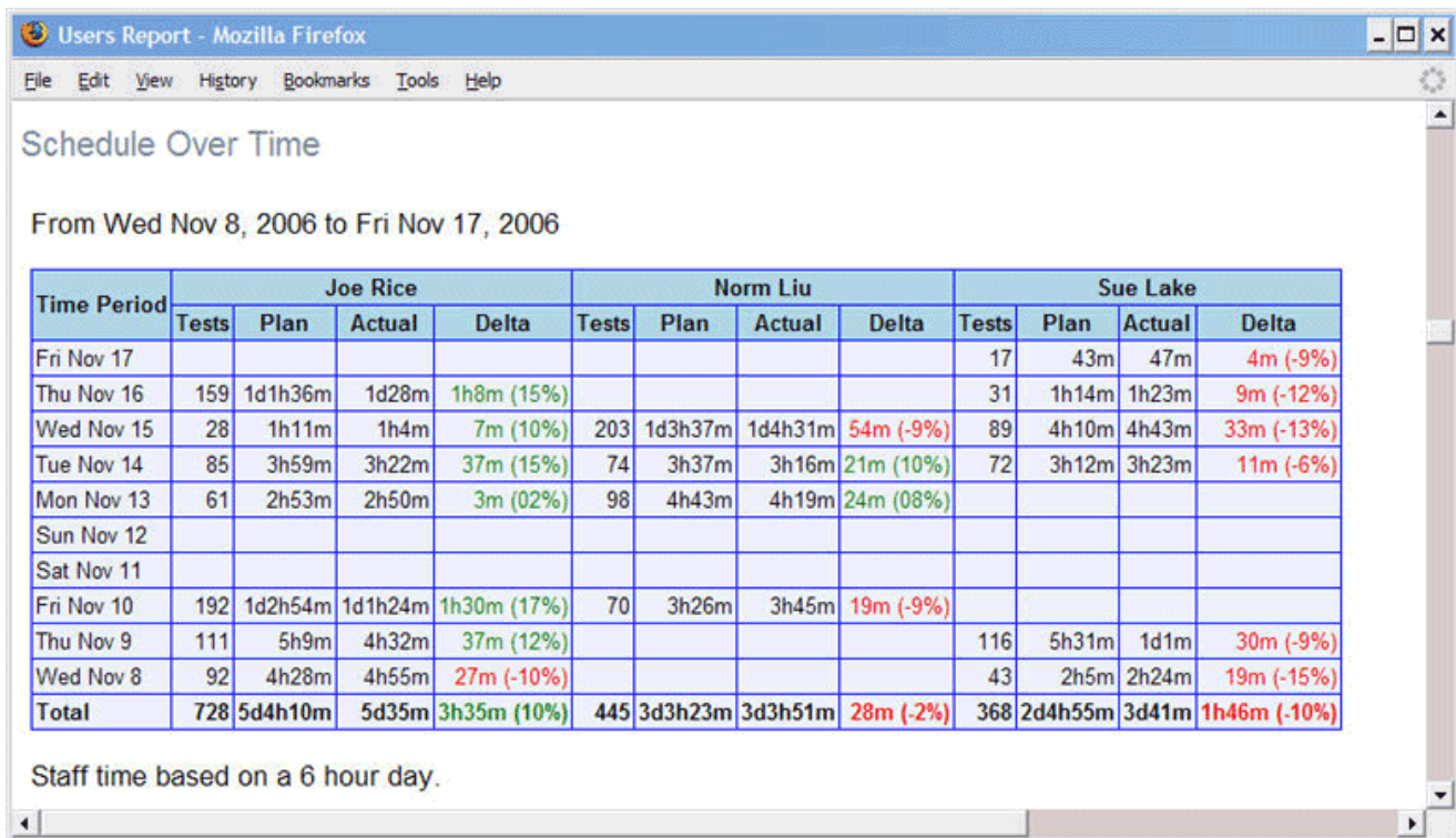
Figure 26 - Users Report
