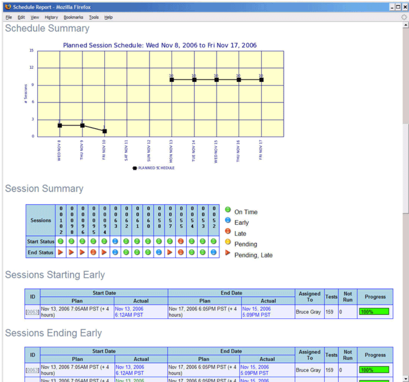
Figure 29 - Schedule Report
