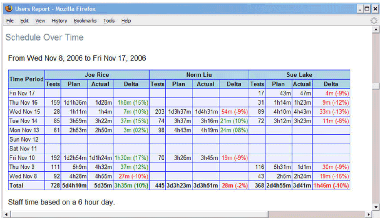
Figure 26 - Users Report
