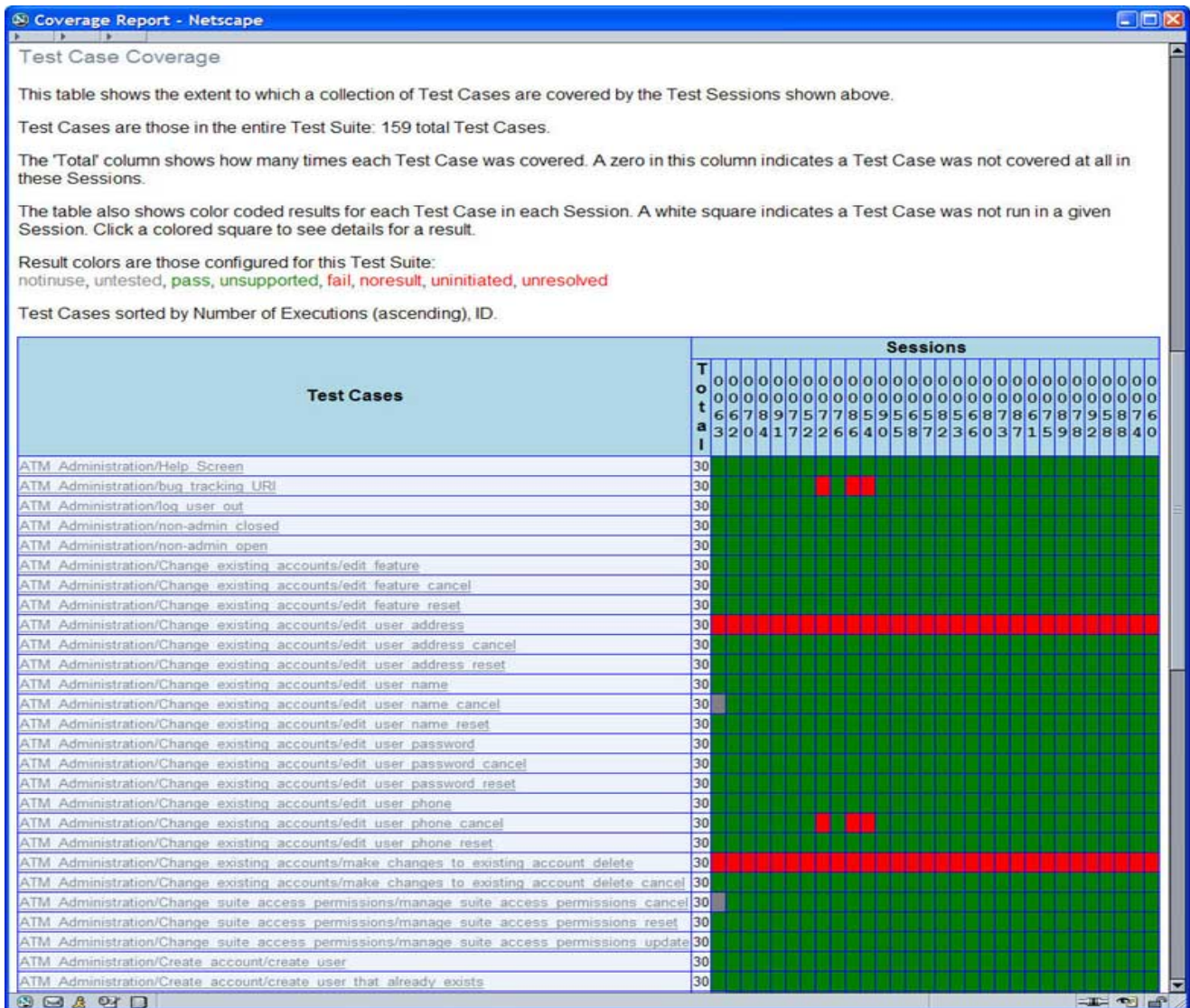
Figure 28 - Coverage Report
