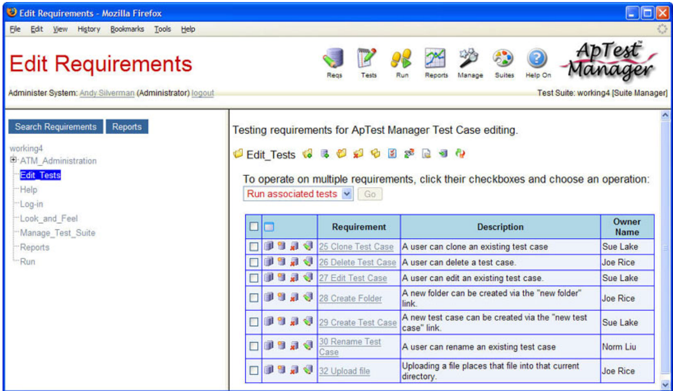
Figure 14 - Requirements tree
