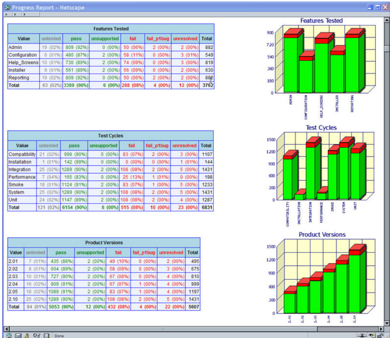
Figure 18 - Selector Summary Tables
