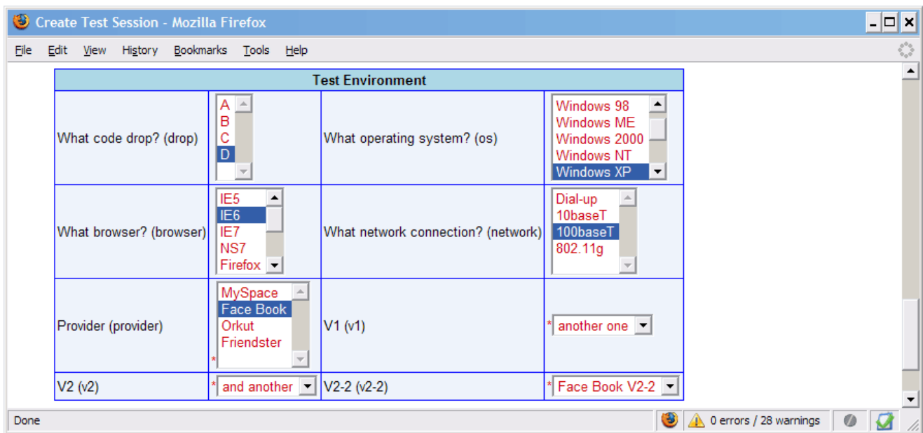
Figure 27 - Session Variable Selections
