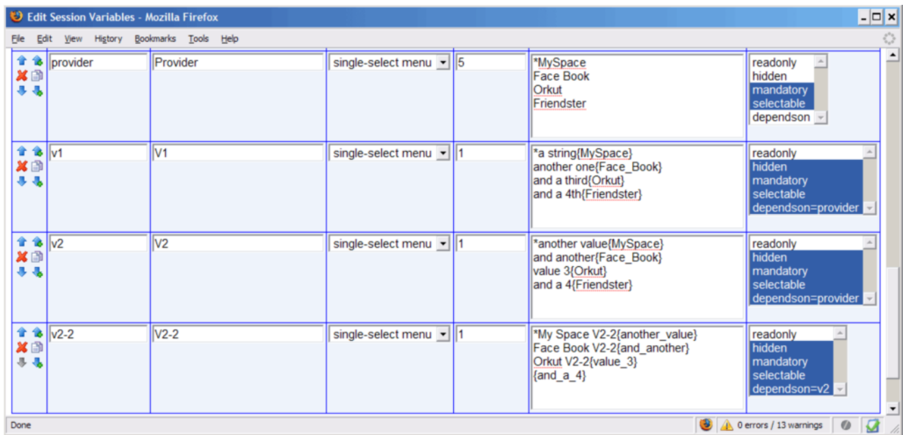
Figure 26 - Parameterization Session Variables
