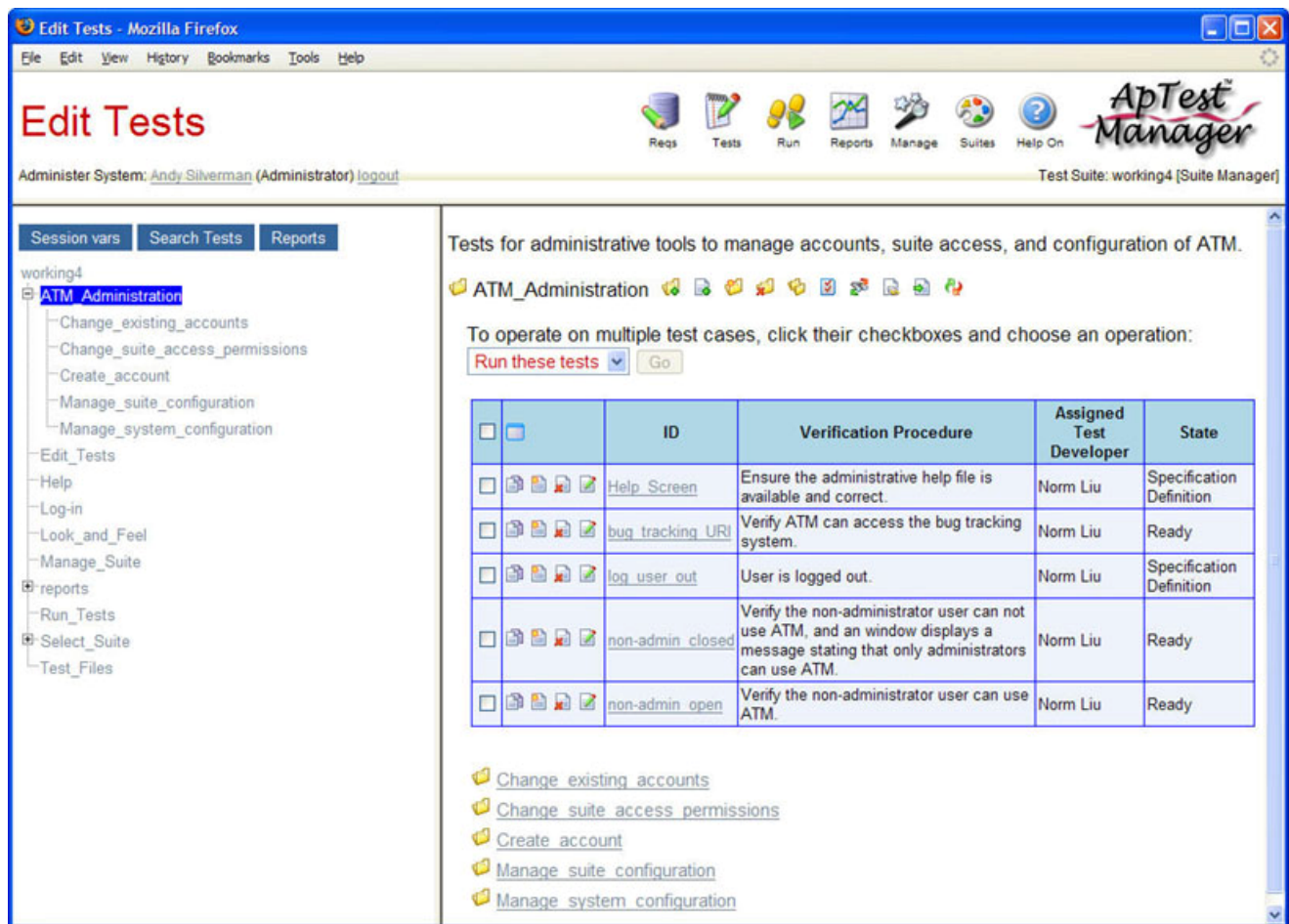
Figure 5 - Test Case tree
