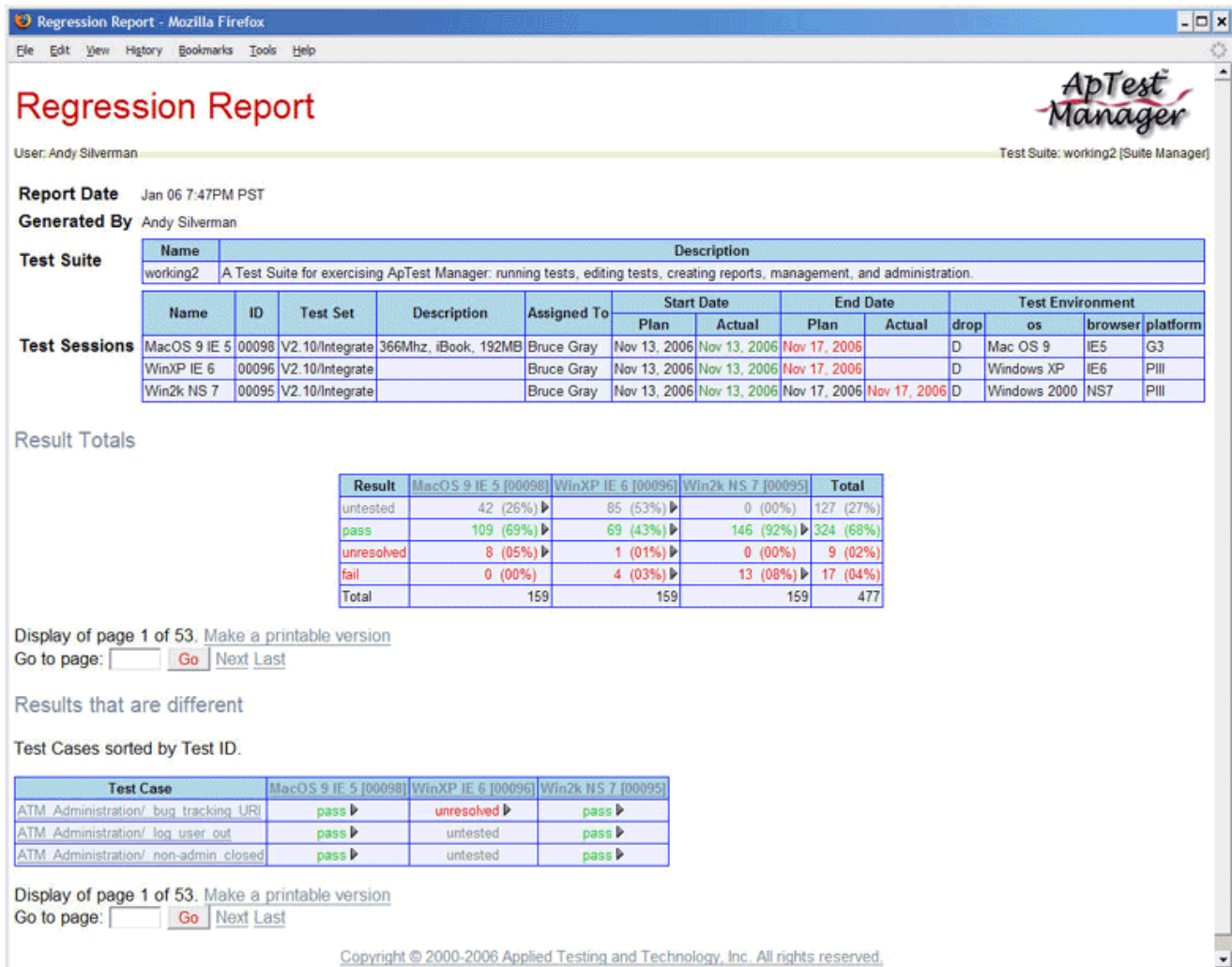
Figure 20 - Regression Report
